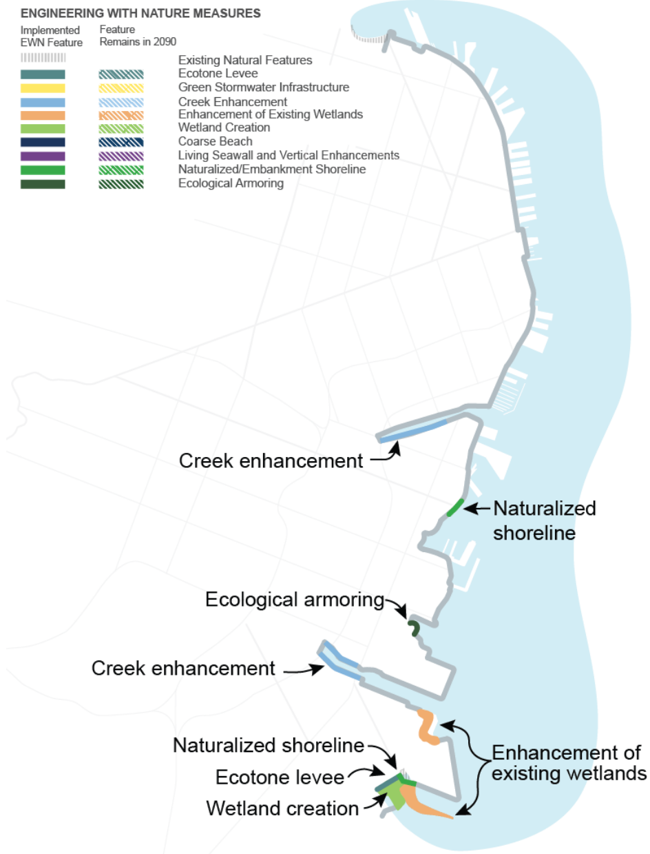
Figure I-36: Natural and Nature-Based Features in Alternative G (2040)
