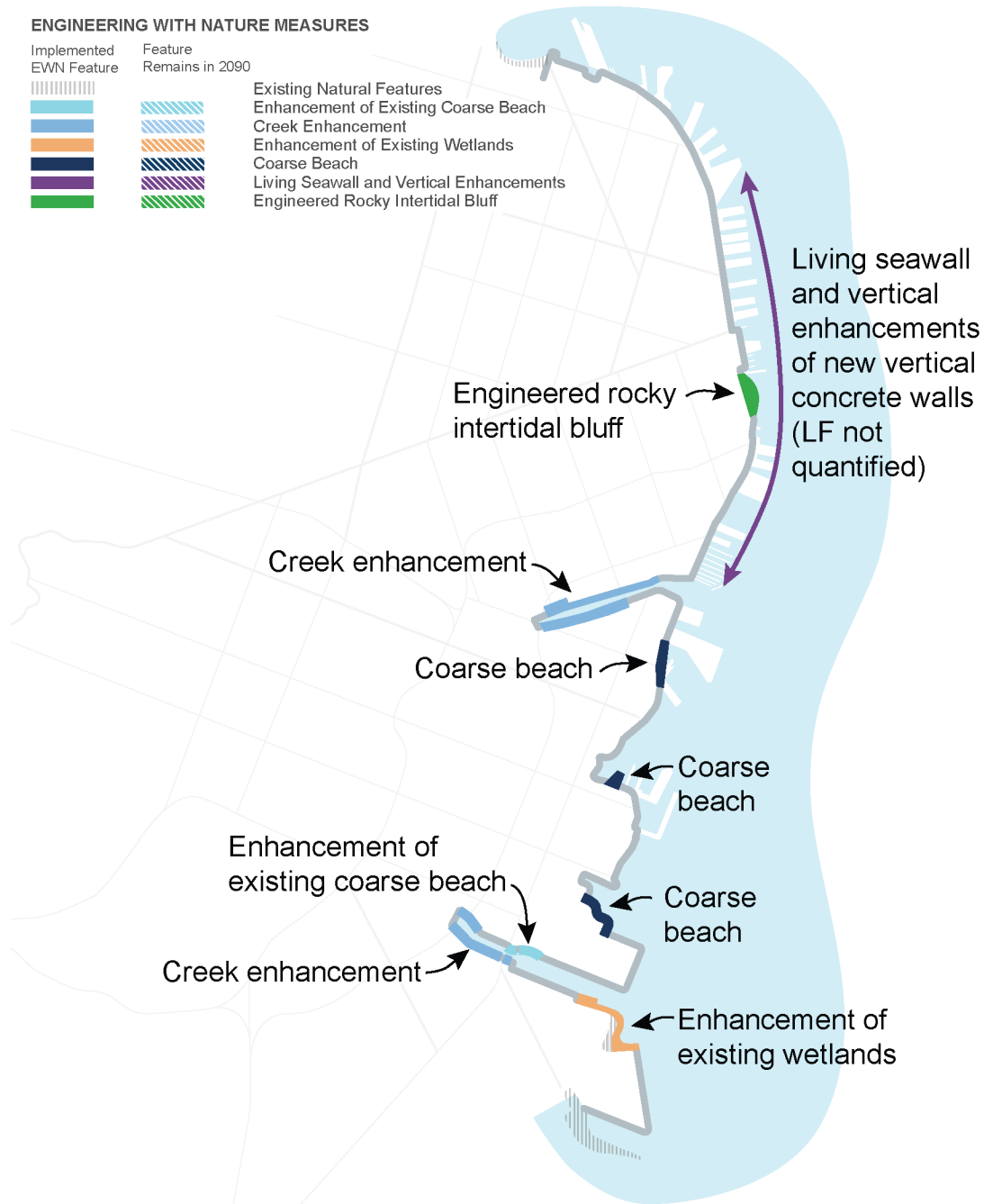
Figure I-38: Natural and Nature-Based Features in the Recommended Plan
