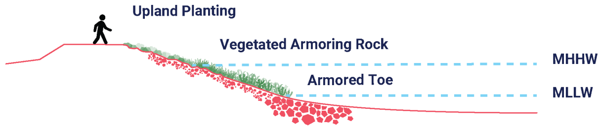
Figure I-21: Schematic of Embankment Shoreline
