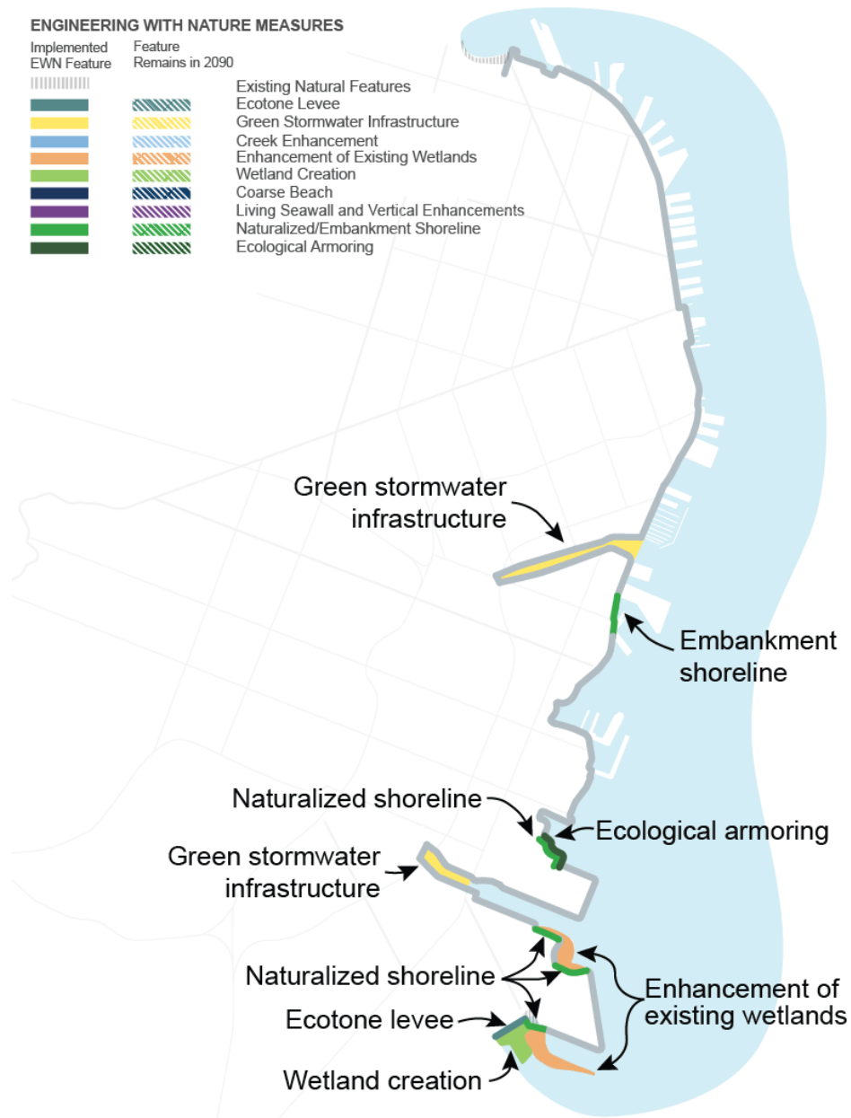
Figure I-34: Natural and Nature-Based Features in Alternative F (2040)
