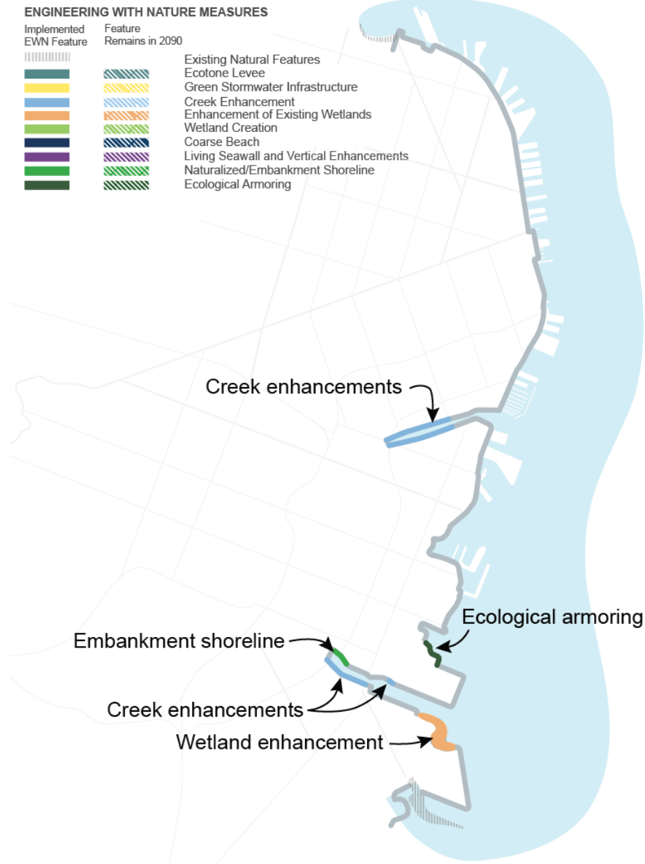
Figure I-29: Natural and Nature-Based Features in Alternative C
