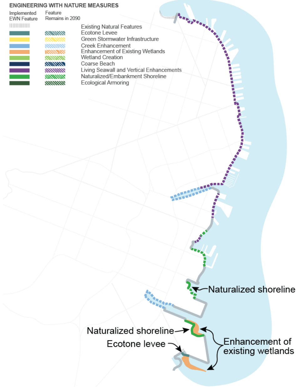
Figure I-33: Natural and Nature-Based Features in Alternative E (2090)
