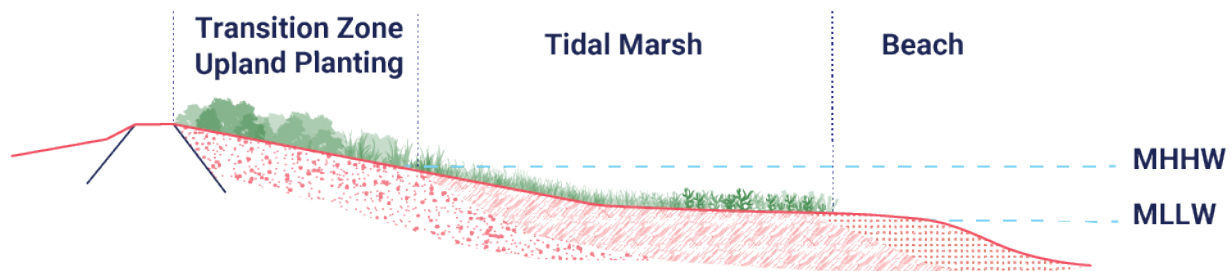
Figure I-13: Schematic of Ecotone Levee
